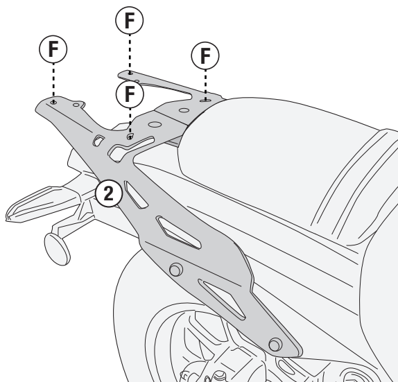
M8 PLATE
